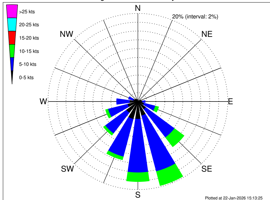
Liberia MBES Climatological Wind Rose for May: 1979 - 2015
