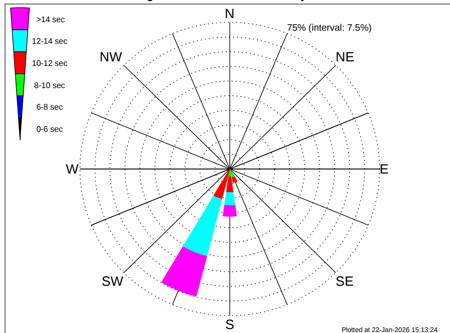
Liberia MBES Climatological WavePeriod Rose for May: 1979 - 2015
