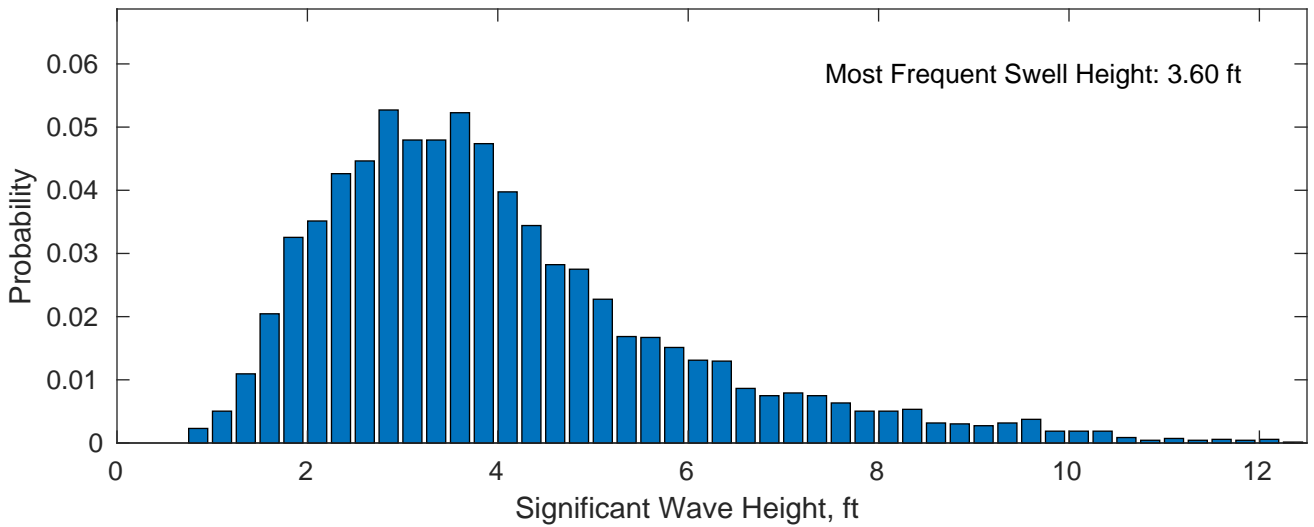
Swell: 74.86%
