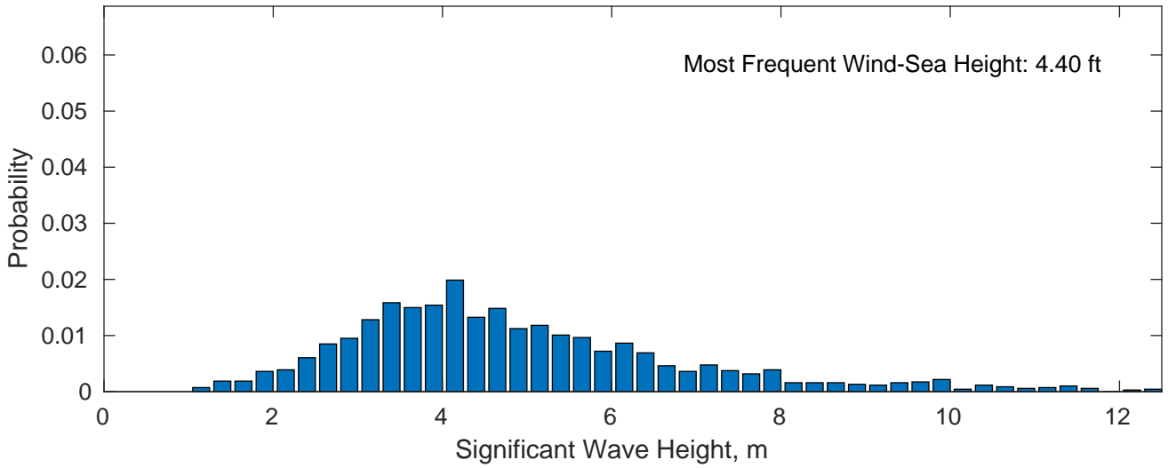
Wind-Sea: 25.14%
