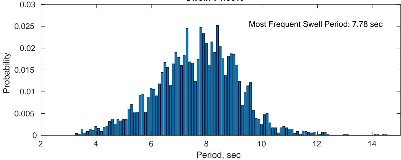
Swell: 74.86%
