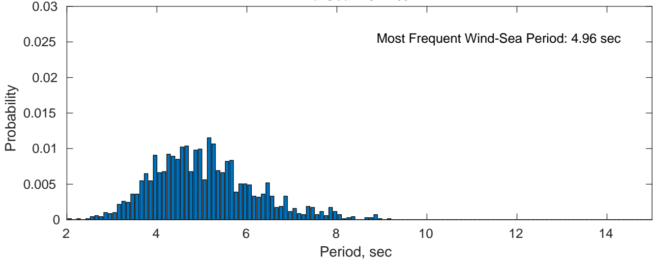
Wind-Sea: 25.14%
