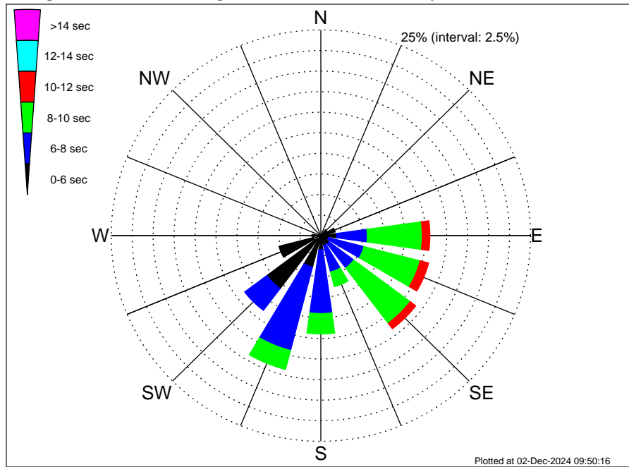
Long Island Wind Climatological WavePeriod Rose for May: 1979 - 2015
