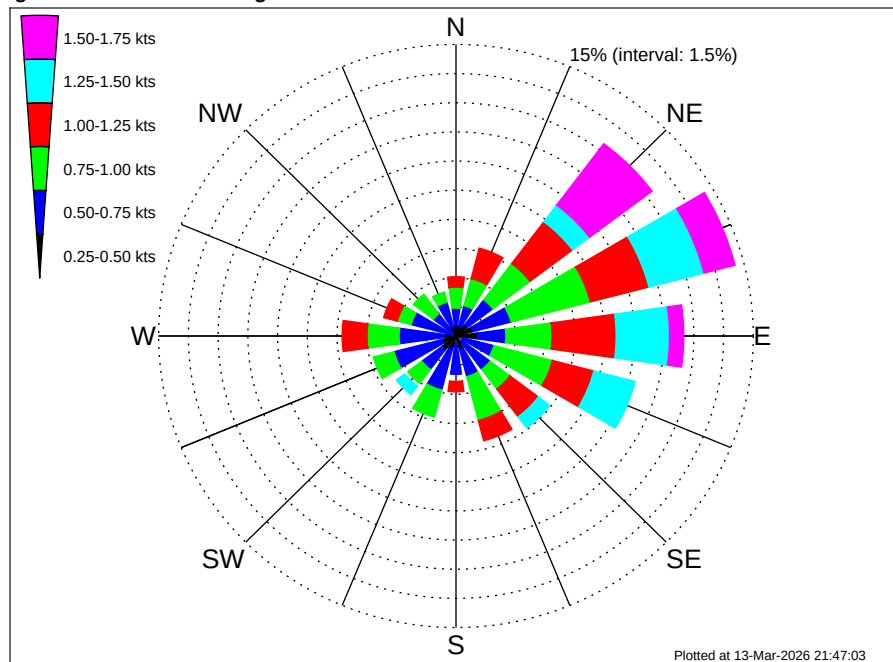
Madagascar MBES Climatological Surface Current Rose for December: 1995 - 2012
