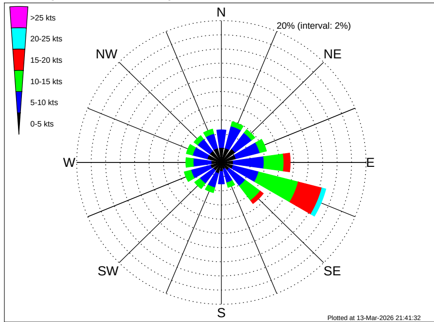
Madagascar MBES Climatological Wind Rose for March: 1979 - 2015
