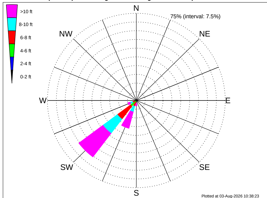
Namibia TE Luderitz (PEL-83) Climatological WaveHeight Rose for April: 1979 - 2015
