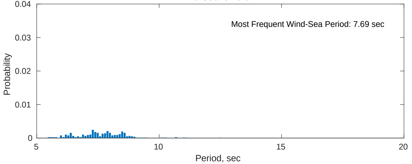
Wind-Sea: 3.46%
