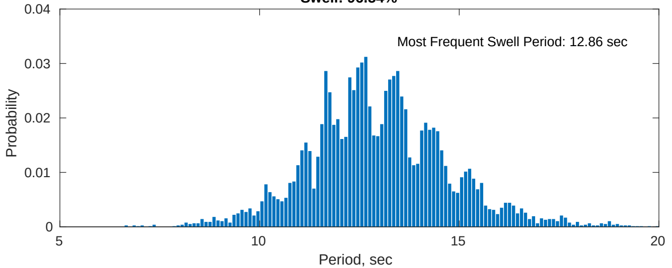
Swell: 96.54%
