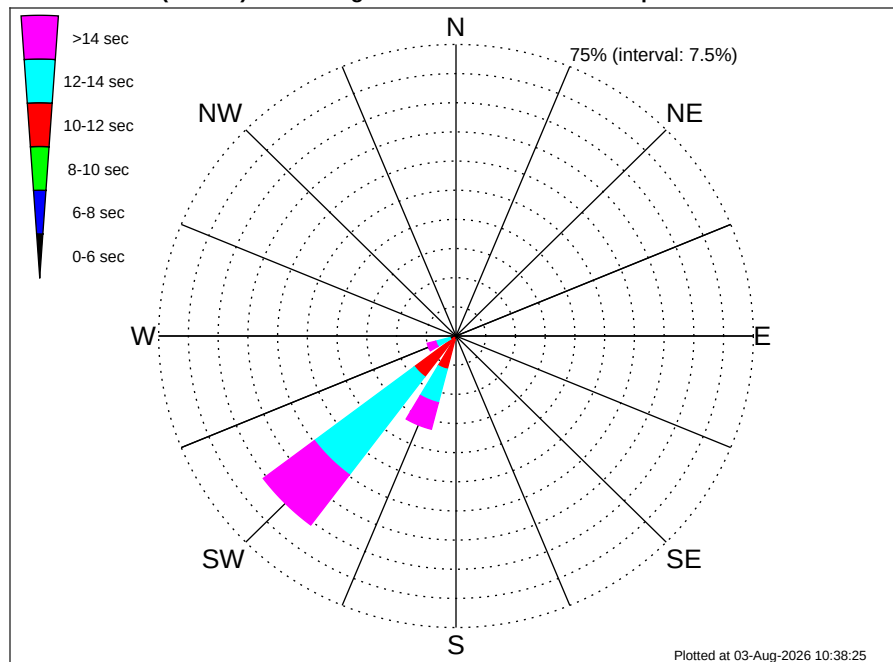
Namibia TE Luderitz (PEL-83) Climatological WavePeriod Rose for April: 1979 - 2015
