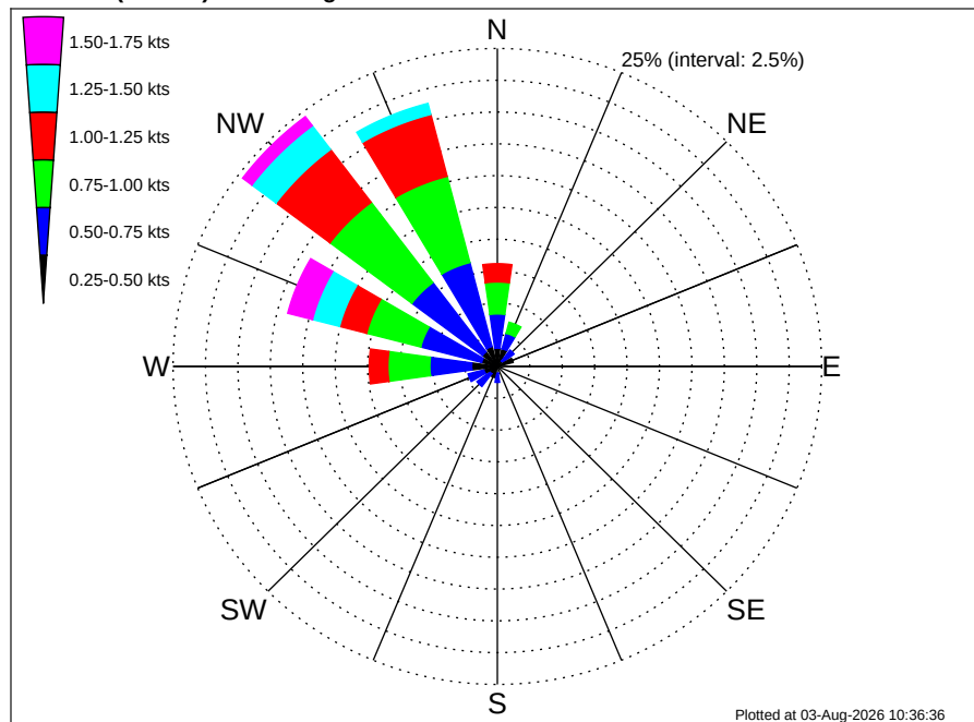
Namibia TE Luderitz (PEL-83) Climatological Surface Current Rose for December: 1995 - 2012
