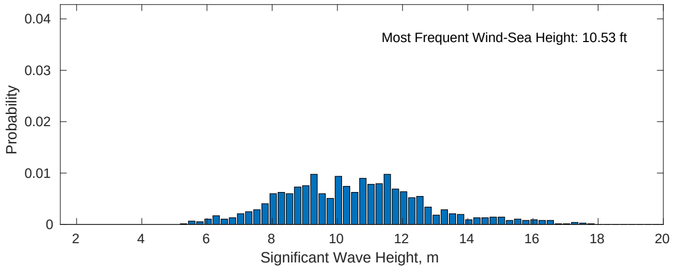
Wind-Sea: 17.77%
