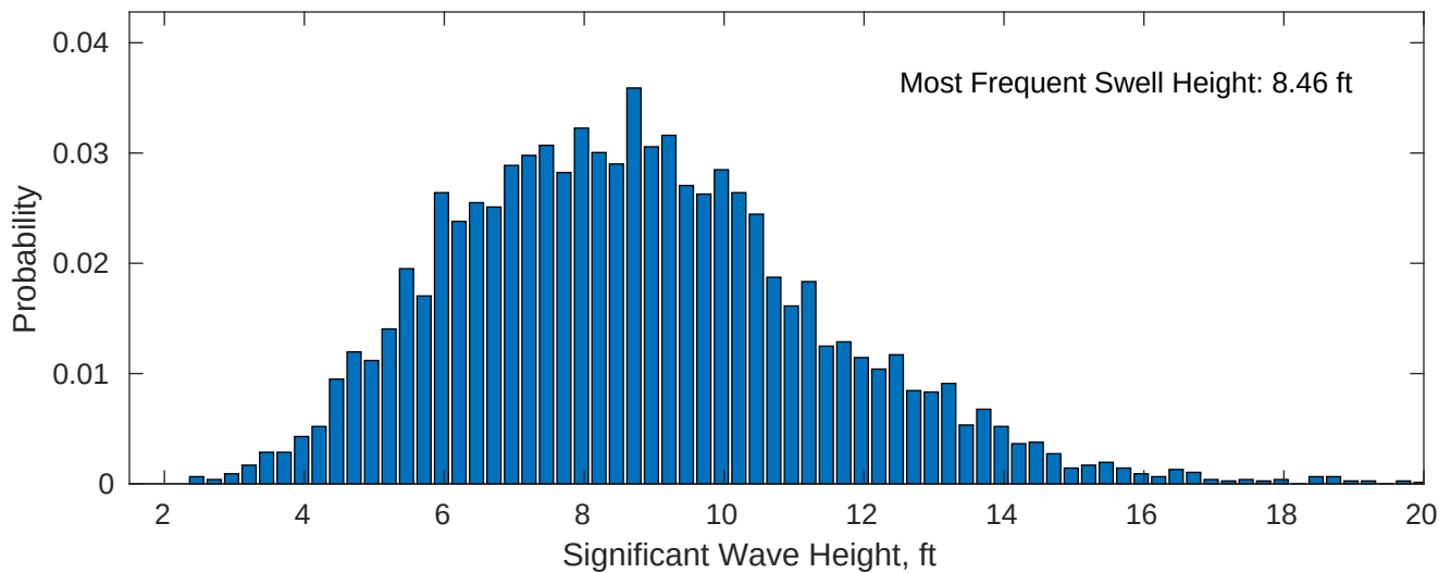
Swell: 82.23%
