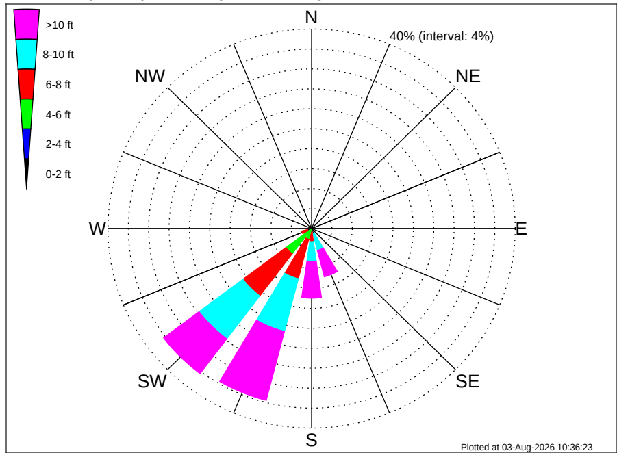
Namibia TE Luderitz (PEL-83) Climatological WaveHeight Rose for December: 1979 - 2015
