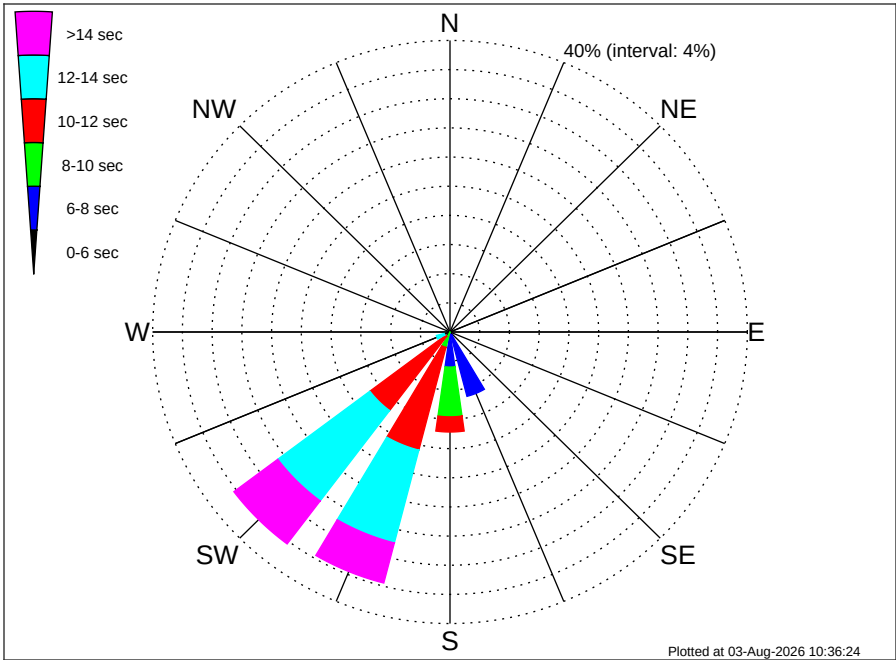
Namibia TE Luderitz (PEL-83) Climatological WavePeriod Rose for December: 1979 - 2015
