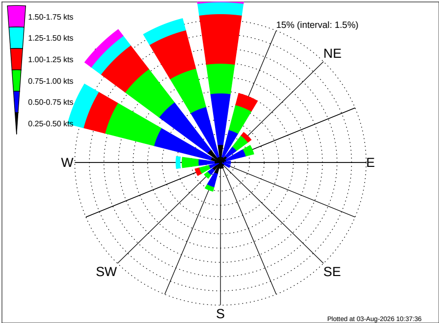
Namibia TE Luderitz (PEL-83) Climatological Surface Current Rose for February: 1995 - 2012
