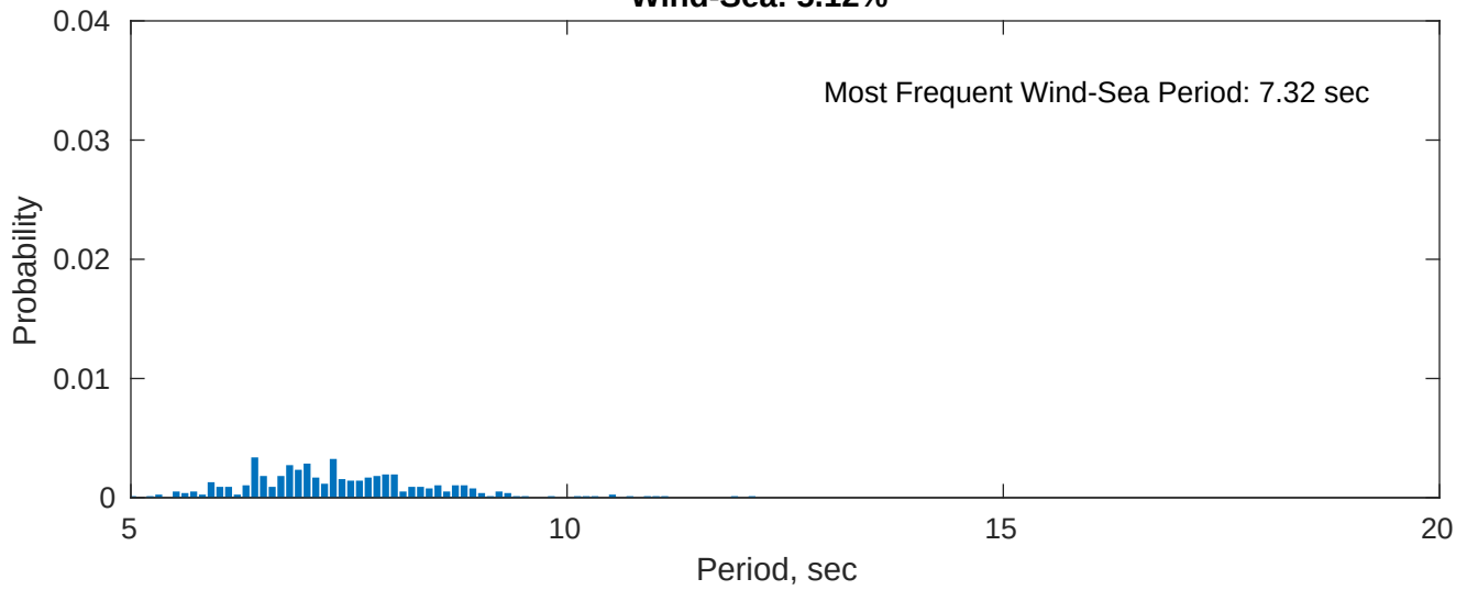
Wind-Sea: 5.12%
