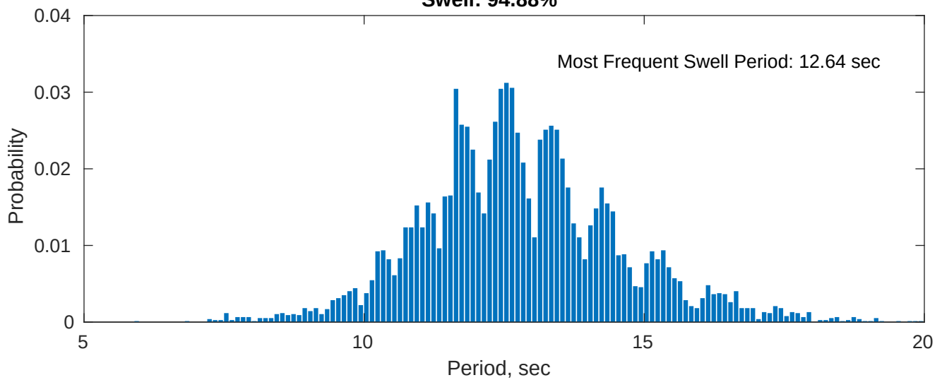
Swell: 94.88%
