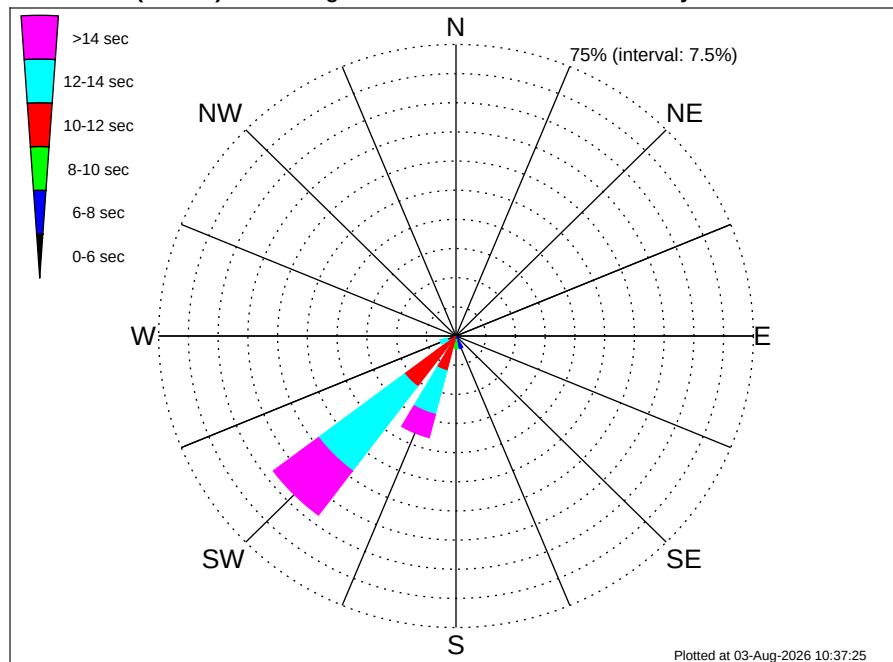
Namibia TE Luderitz (PEL-83) Climatological WavePeriod Rose for February: 1979 - 2015
