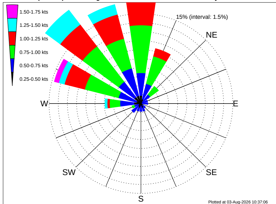
Namibia TE Luderitz (PEL-83) Climatological Surface Current Rose for January: 1995 - 2012
