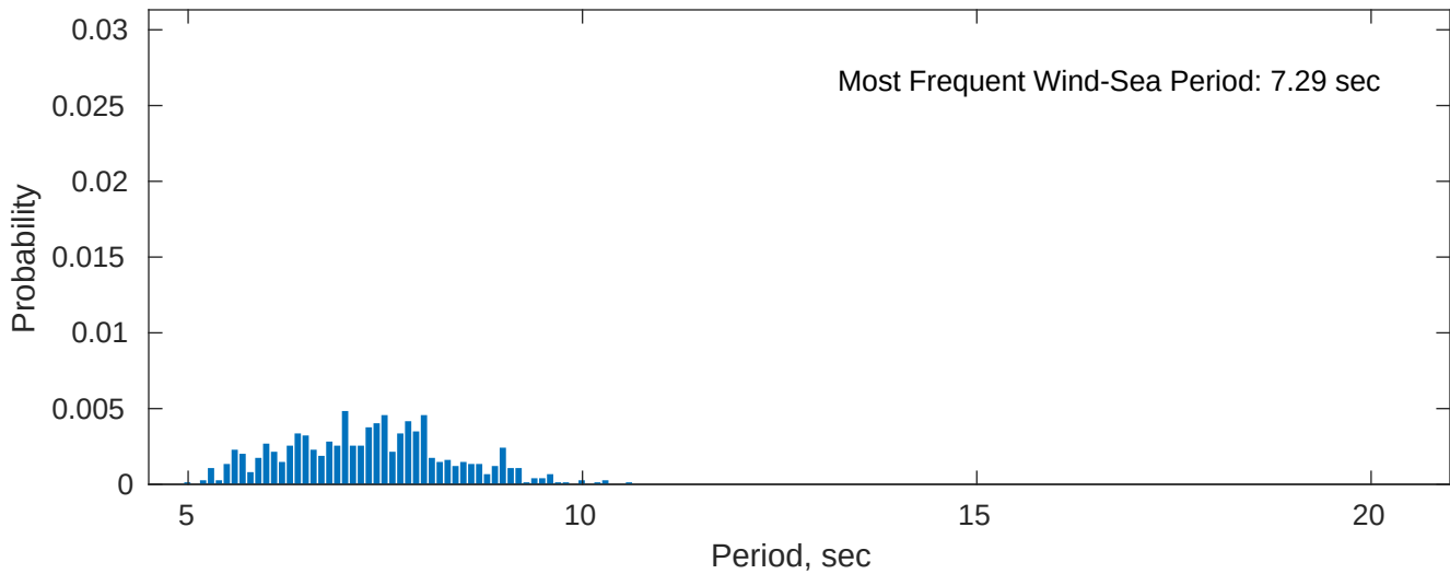
Wind-Sea: 9.44%
