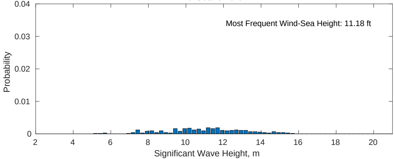
Wind-Sea: 3.20%
