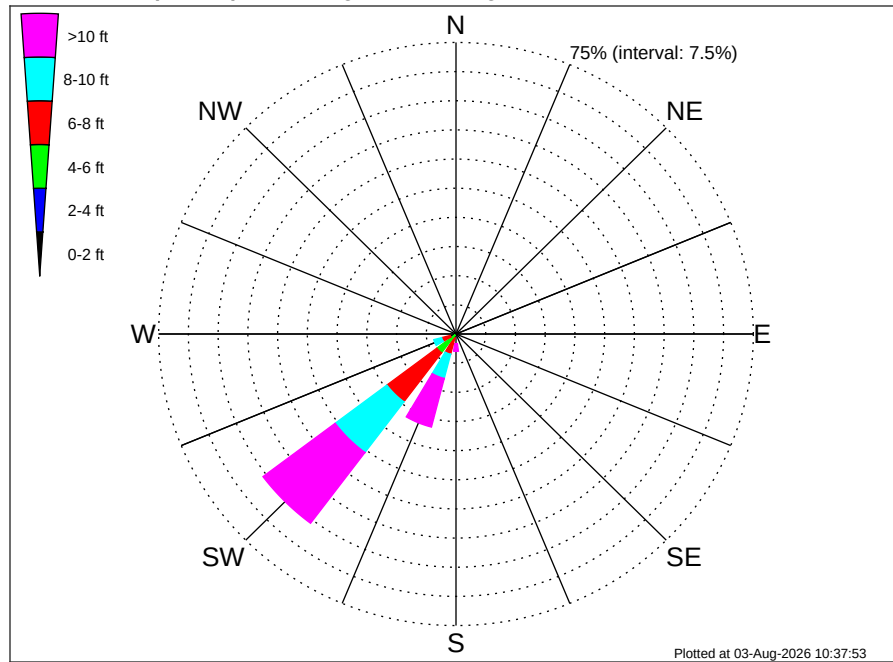
Namibia TE Luderitz (PEL-83) Climatological WaveHeight Rose for March: 1979 - 2015
