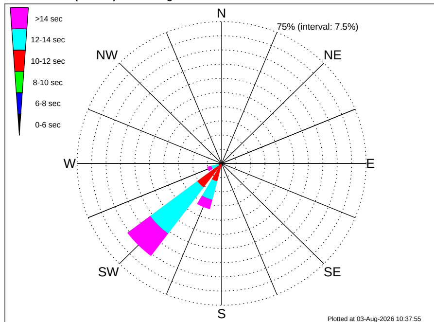
Namibia TE Luderitz (PEL-83) Climatological WavePeriod Rose for March: 1979 - 2015
