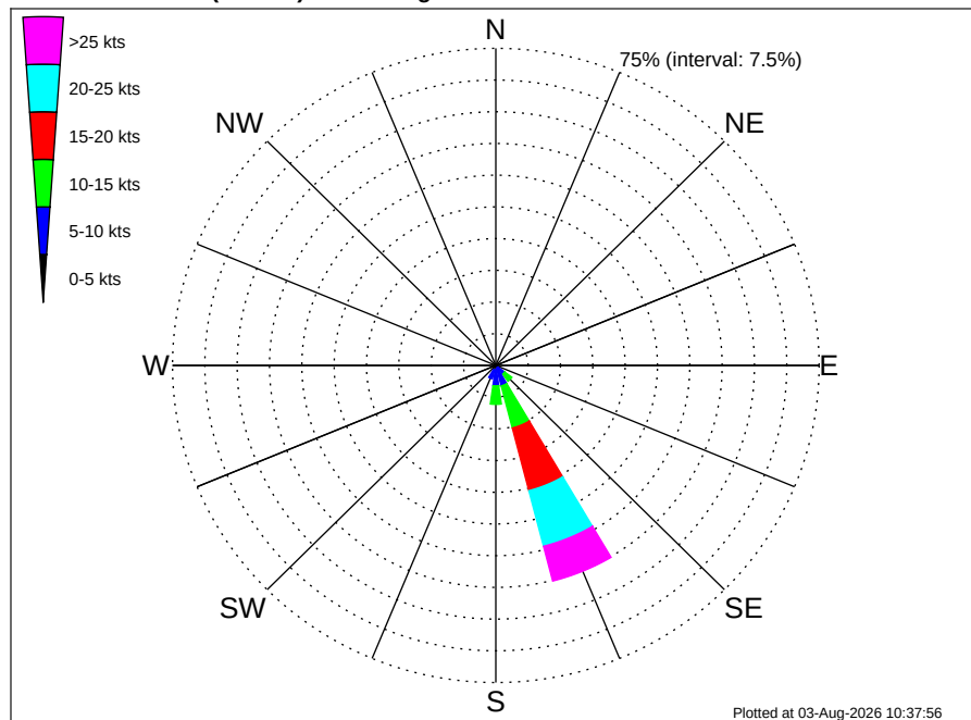
Namibia TE Luderitz (PEL-83) Climatological Wind Rose for March: 1979 - 2015
