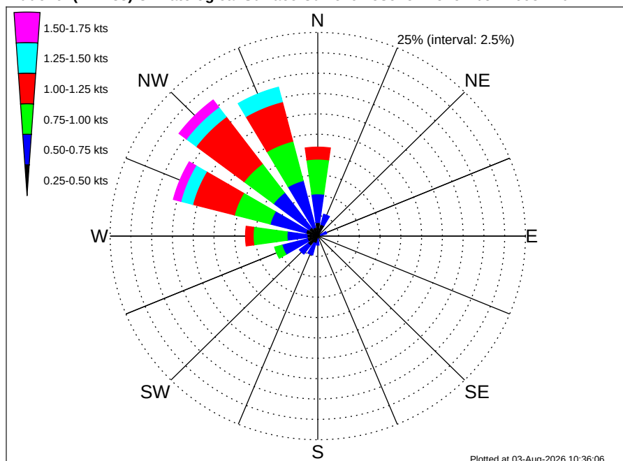
Namibia TE Luderitz (PEL-83) Climatological Surface Current Rose for November: 1995 - 2012
