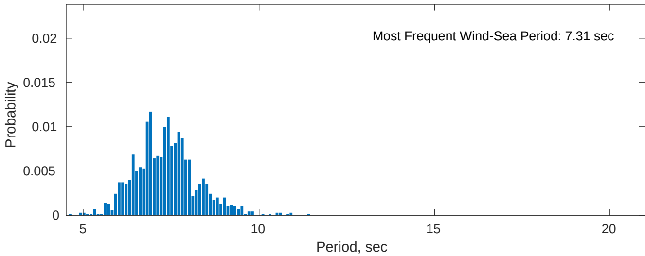
Wind-Sea: 18.79%
