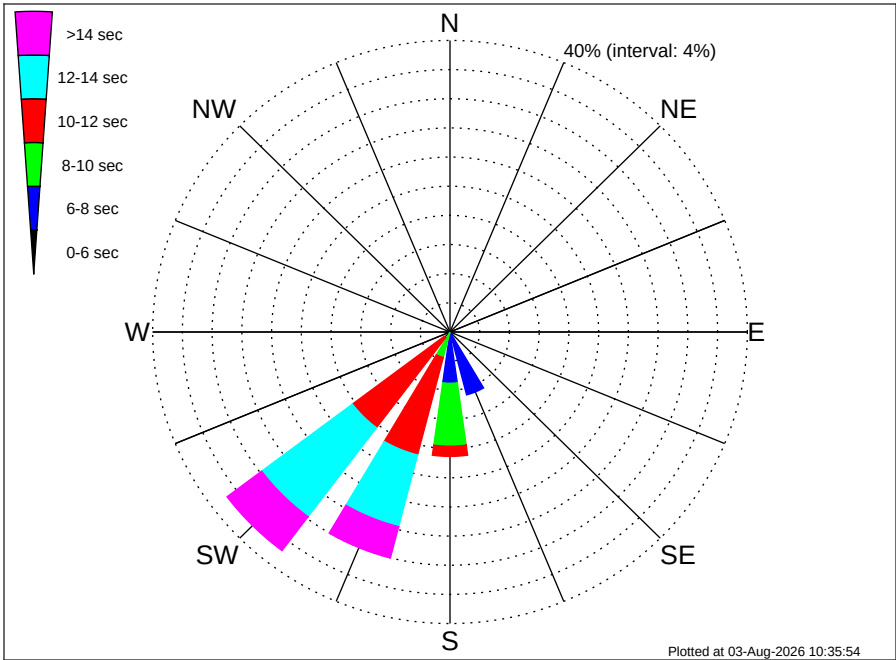
Namibia TE Luderitz (PEL-83) Climatological WavePeriod Rose for November: 1979 - 2015
