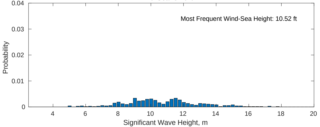
Wind-Sea: 5.46%
