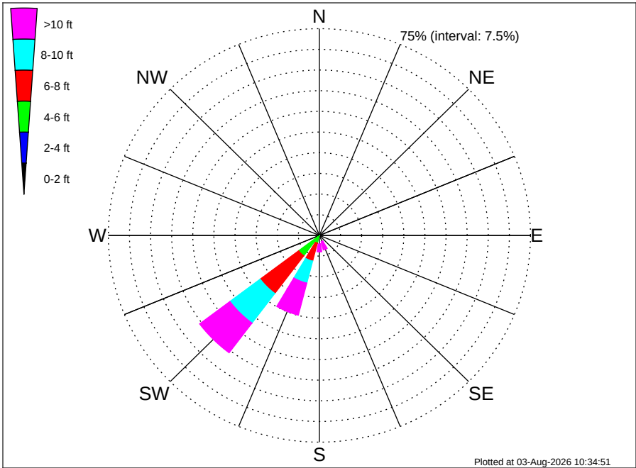
Namibia TE Oranjemund (PEL-104) Climatological WaveHeight Rose for April: 1979 - 2015
