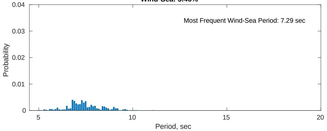
Wind-Sea: 5.46%
