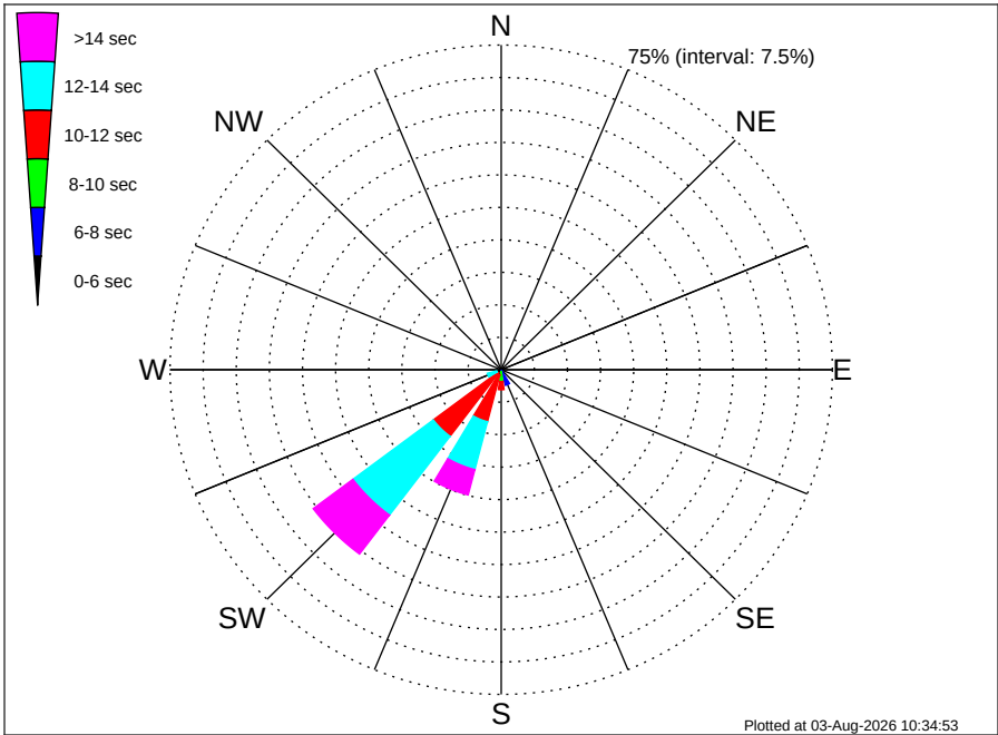
Namibia TE Oranjemund (PEL-104) Climatological WavePeriod Rose for April: 1979 - 2015
