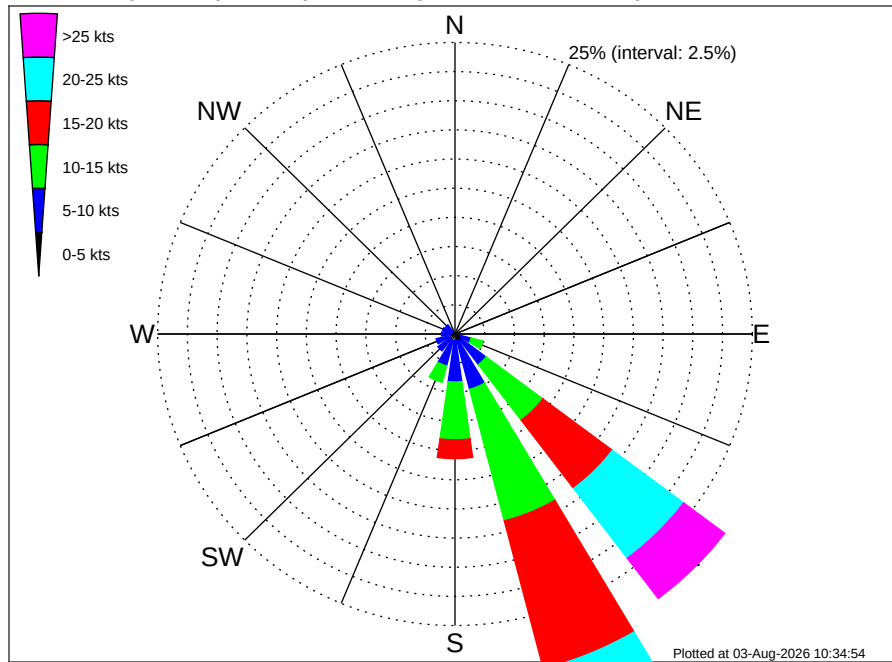
Namibia TE Oranjemund (PEL-104) Climatological Wind Rose for April: 1979 - 2015
