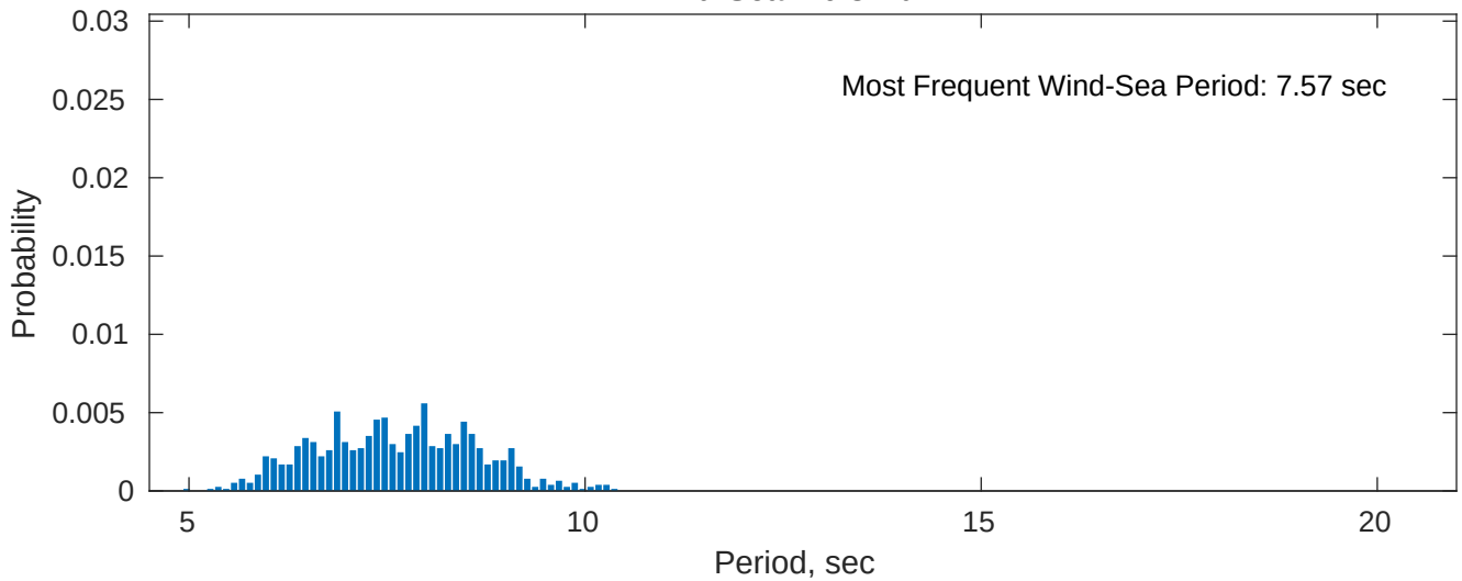
Wind-Sea: 10.84%
