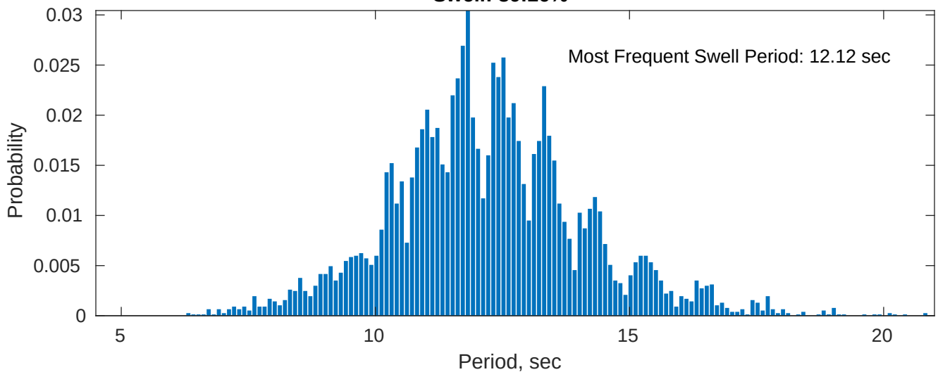
Swell: 89.16%
