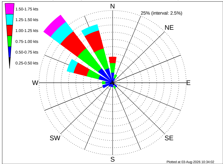
Namibia TE Oranjemund (PEL-104) Climatological Surface Current Rose for February: 1995 - 2012
