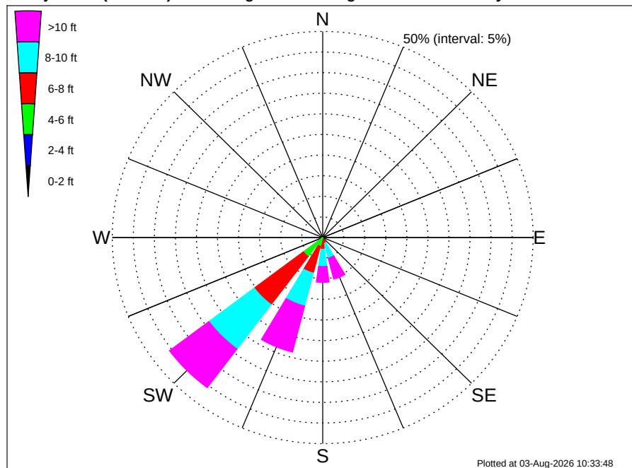
Namibia TE Oranjemund (PEL-104) Climatological WaveHeight Rose for February: 1979 - 2015
