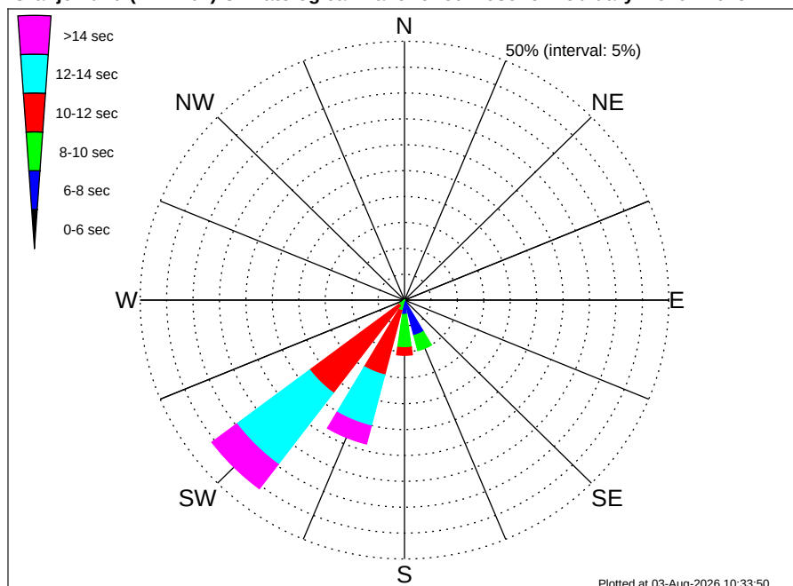
Namibia TE Oranjemund (PEL-104) Climatological WavePeriod Rose for February: 1979 - 2015
