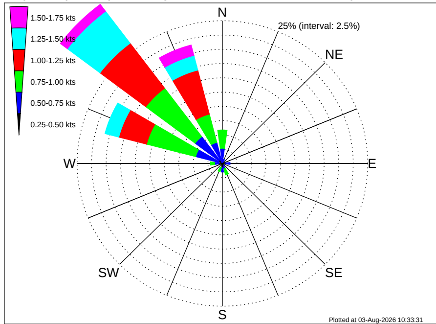
Namibia TE Oranjemund (PEL-104) Climatological Surface Current Rose for January: 1995 - 2012
