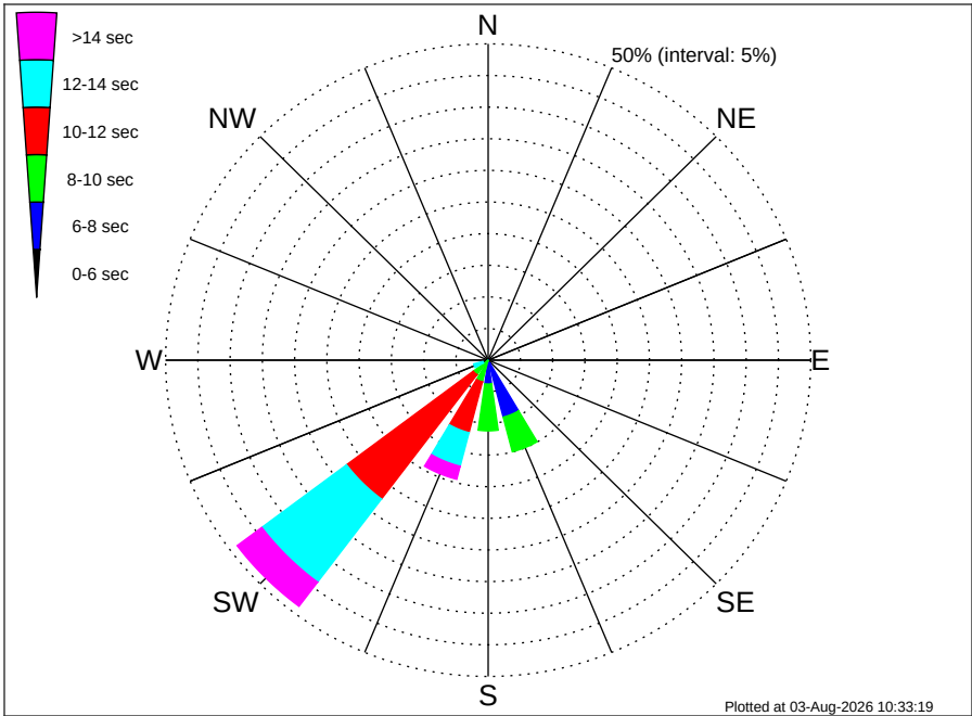
Namibia TE Oranjemund (PEL-104) Climatological WavePeriod Rose for January: 1979 - 2015
