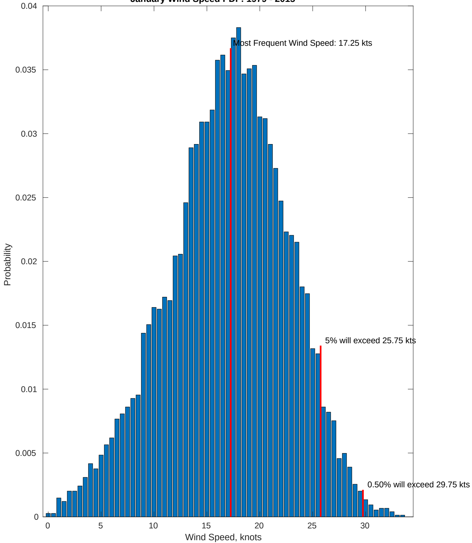
January Wind Speed PDF: 1979 - 2015
