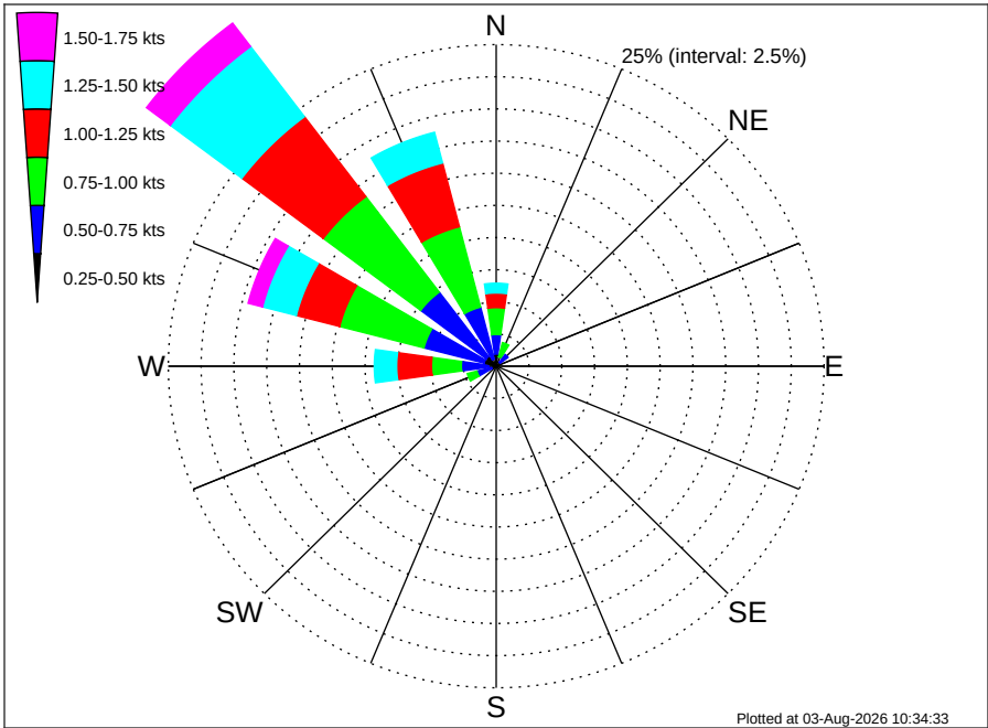
Namibia TE Oranjemund (PEL-104) Climatological Surface Current Rose for March: 1995 - 2012
