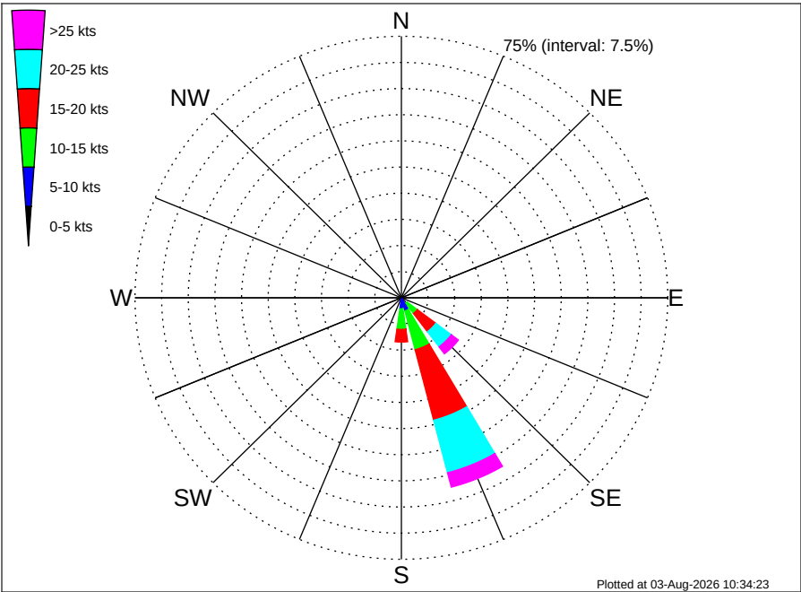
Namibia TE Oranjemund (PEL-104) Climatological Wind Rose for March: 1979 - 2015
