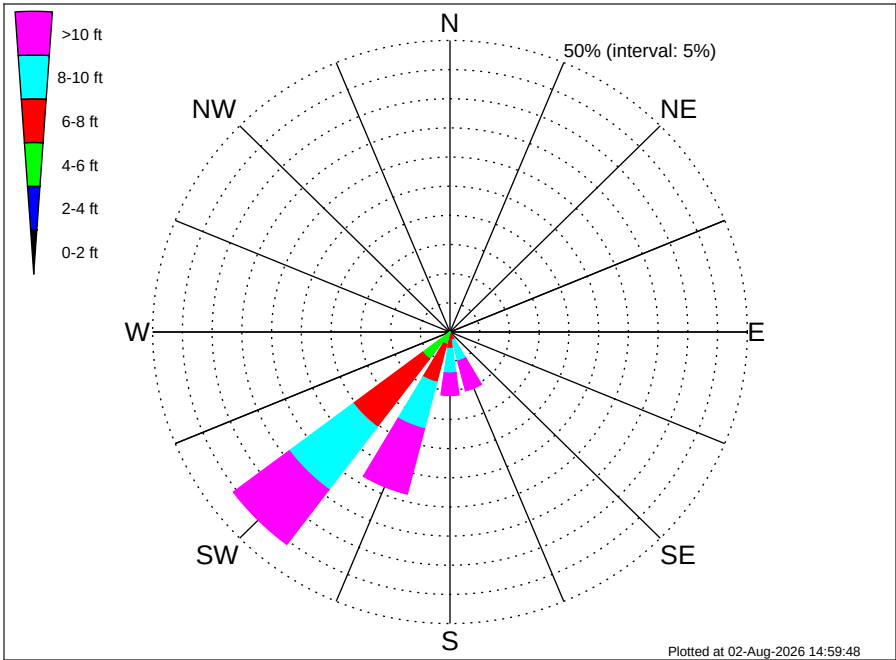
Namibia TE Oranjemund (PEL-104) Climatological WaveHeight Rose for November: 1979 - 2015
