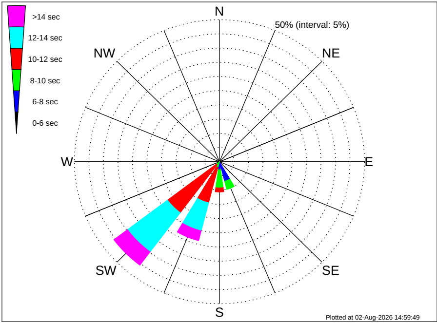
Namibia TE Oranjemund (PEL-104) Climatological WavePeriod Rose for November: 1979 - 2015
