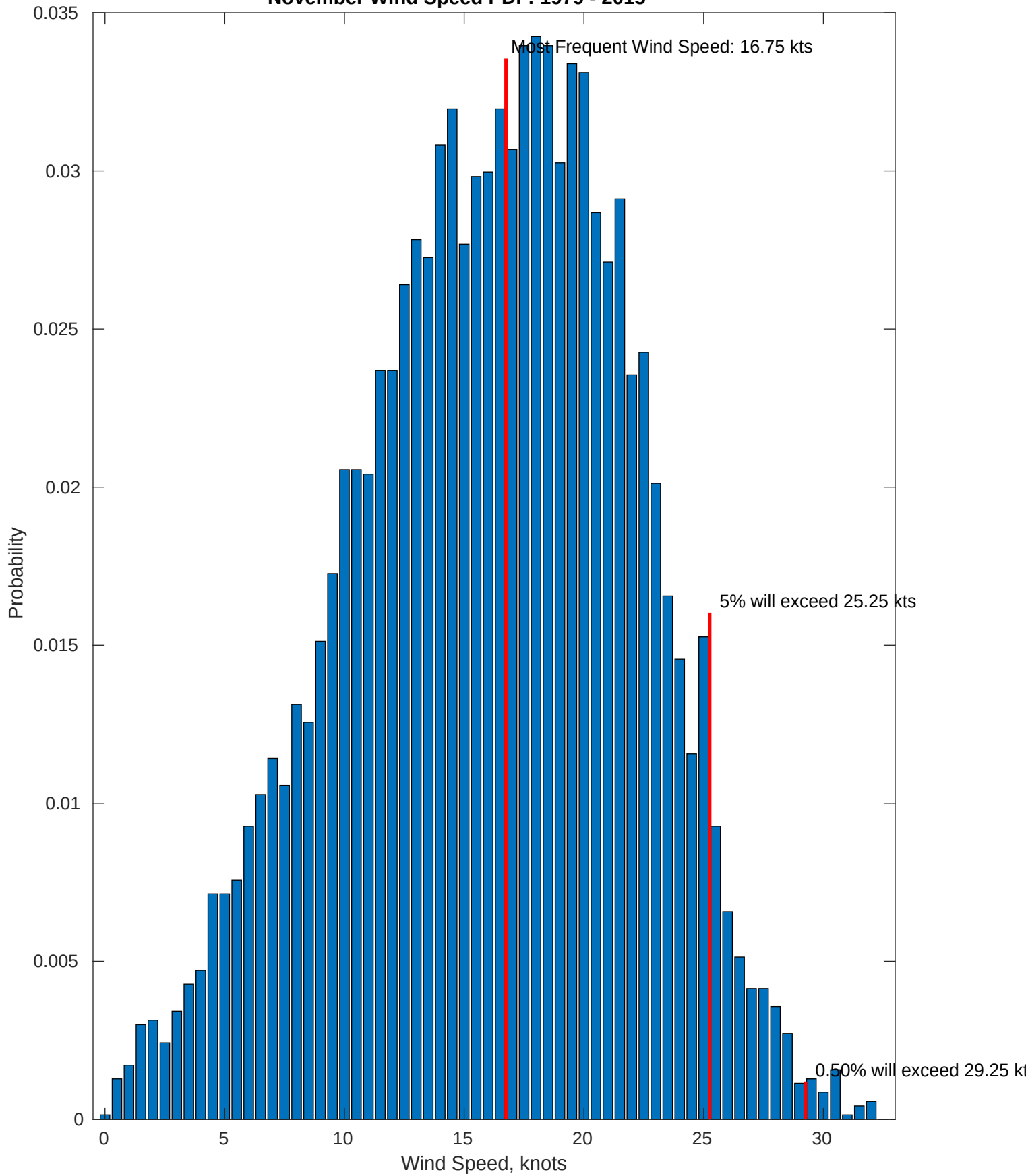
November Wind Speed PDF: 1979 - 2015
