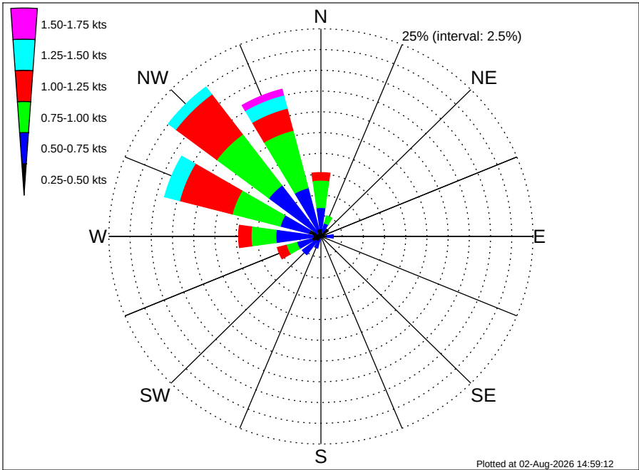
Namibia TE Oranjemund (PEL-104) Climatological Surface Current Rose for October: 1995 - 2012
