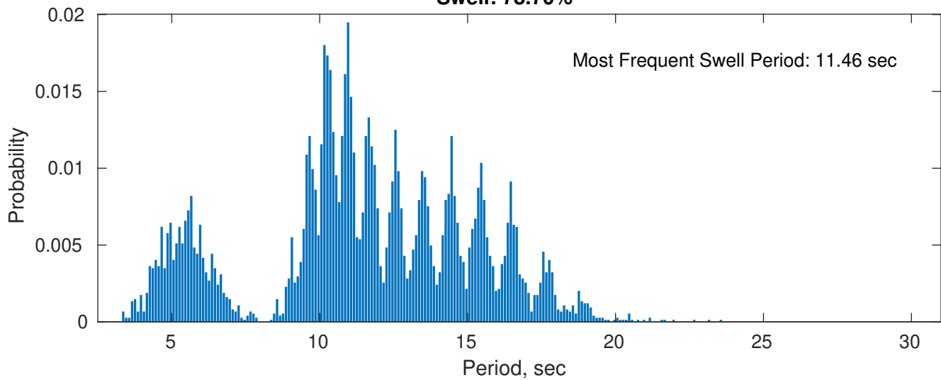
Swell: 78.70%
