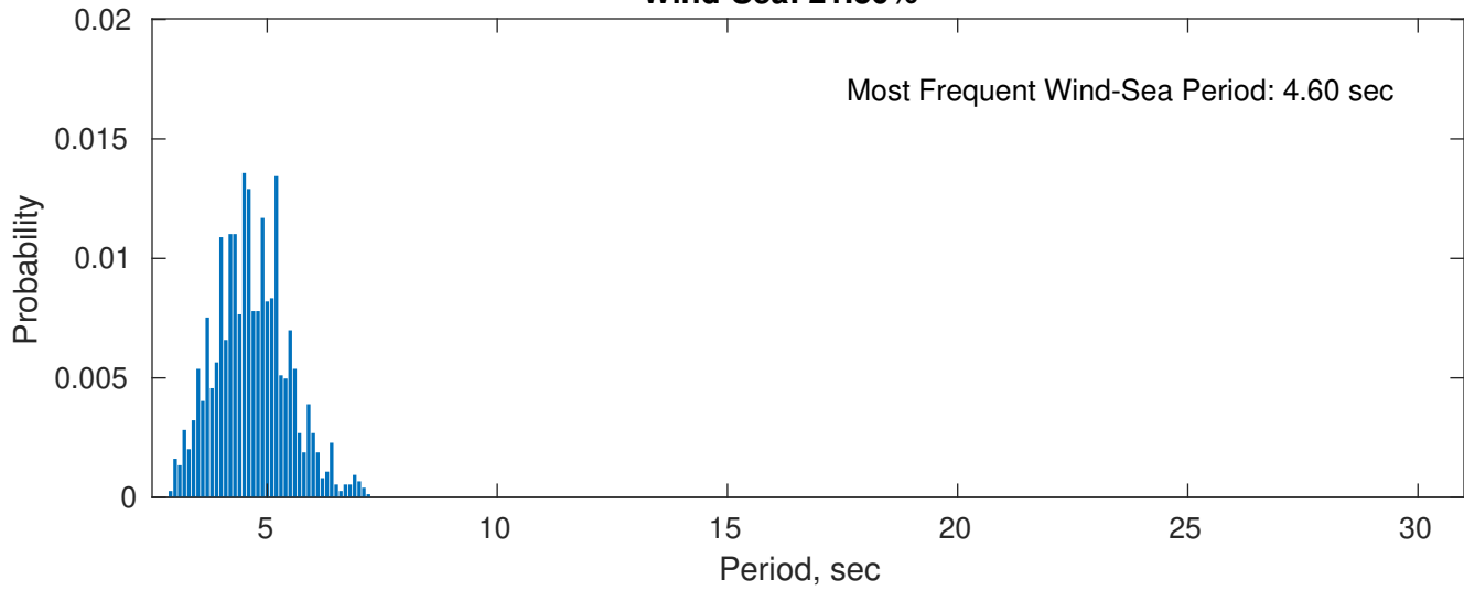
Wind-Sea: 21.30%
