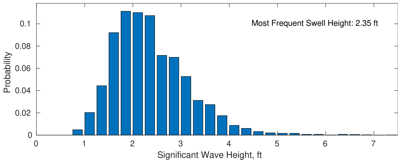
Swell: 78.70%
