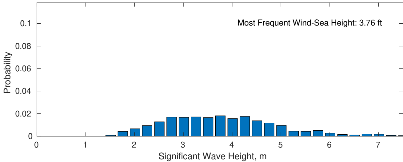
Wind-Sea: 21.30%
