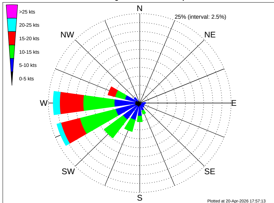
Petronas Oman Block 18 Climatological Wind Rose for April: 1979 - 2015
