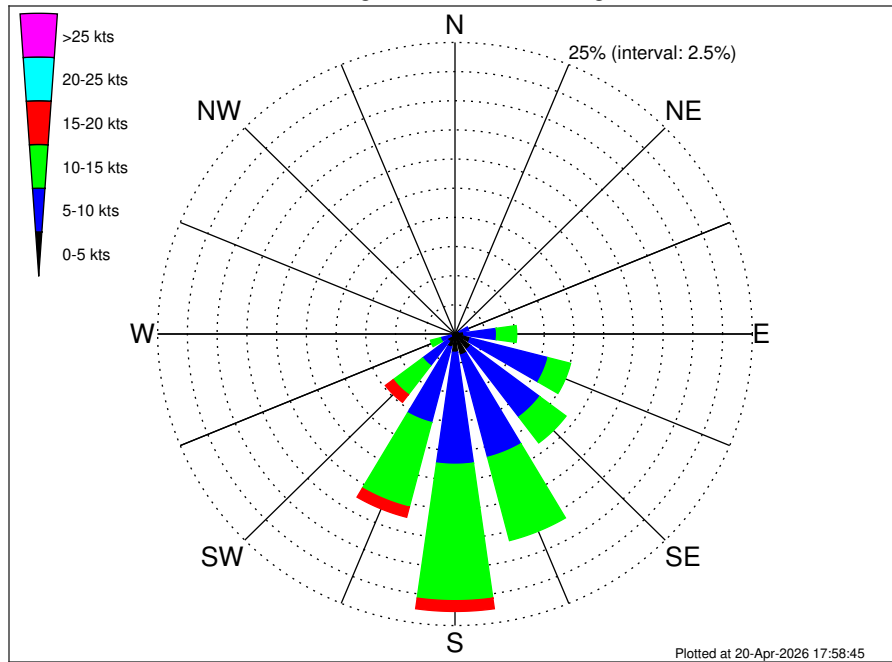
Petronas Oman Block 18 Climatological Wind Rose for August: 1979 - 2015
