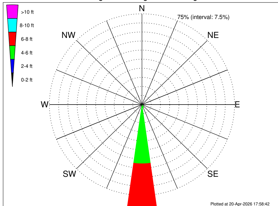
Petronas Oman Block 18 Climatological WaveHeight Rose for August: 1979 - 2015
