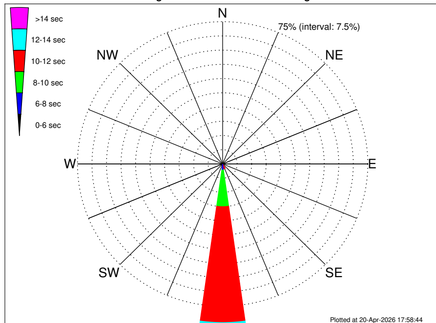
Petronas Oman Block 18 Climatological WavePeriod Rose for August: 1979 - 2015
