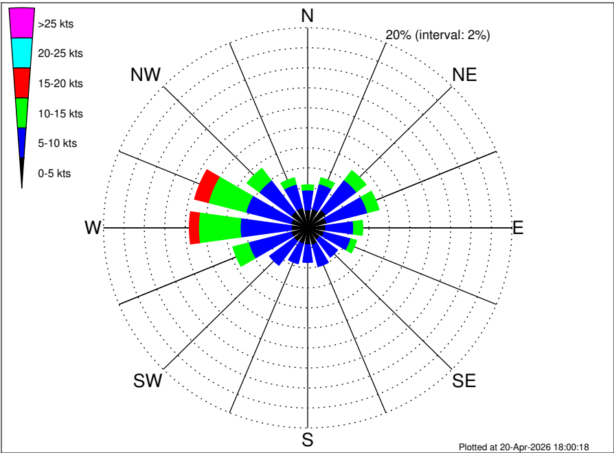
Petronas Oman Block 18 Climatological Wind Rose for December: 1979 - 2015
