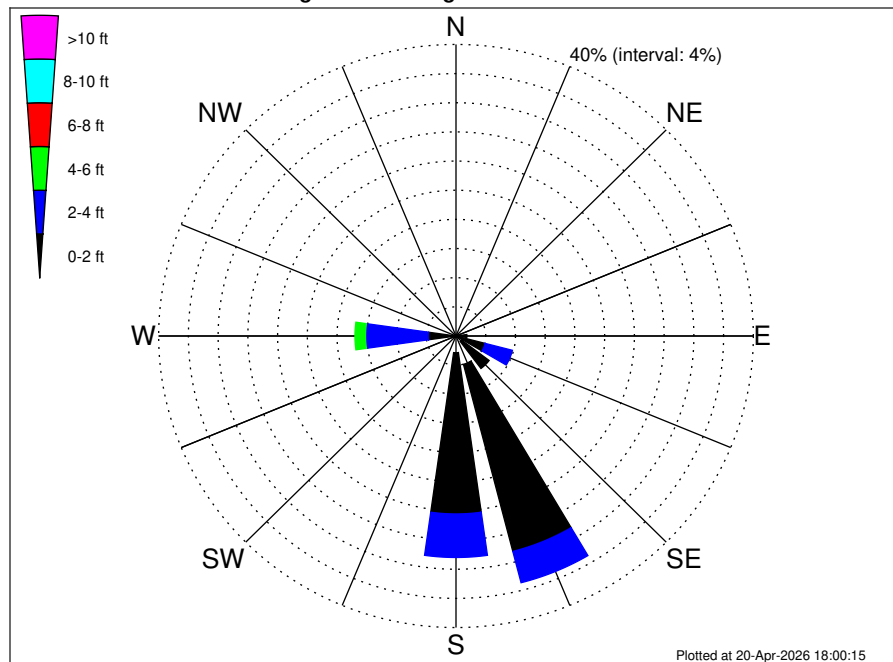
Petronas Oman Block 18 Climatological WaveHeight Rose for December: 1979 - 2015
