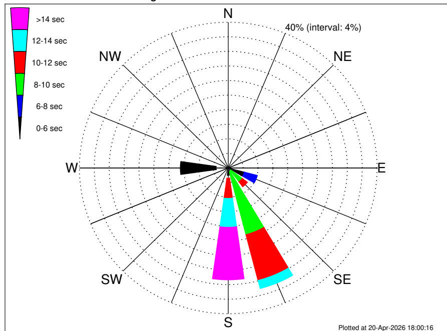
Petronas Oman Block 18 Climatological WavePeriod Rose for December: 1979 - 2015
