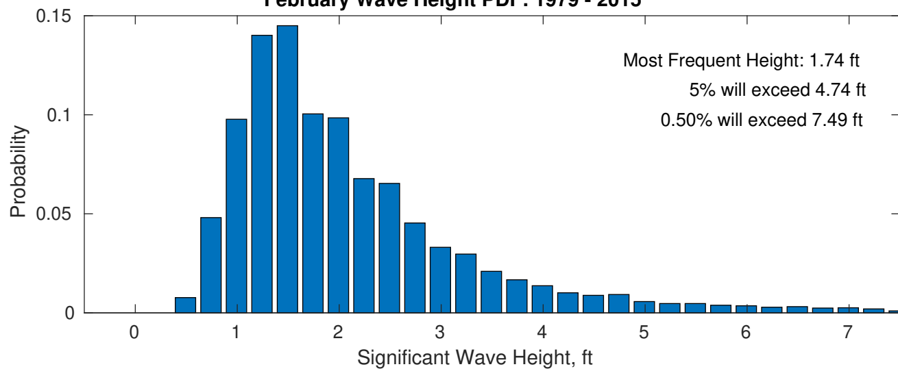
Wind-Sea: 19.19%
