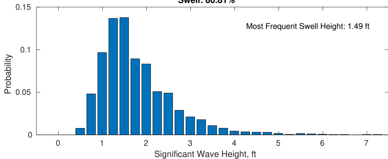
Swell: 80.81%
