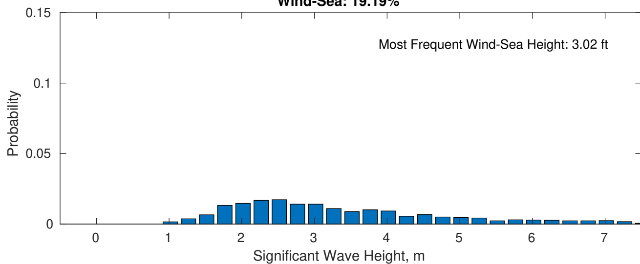
Wind-Sea: 19.19%
