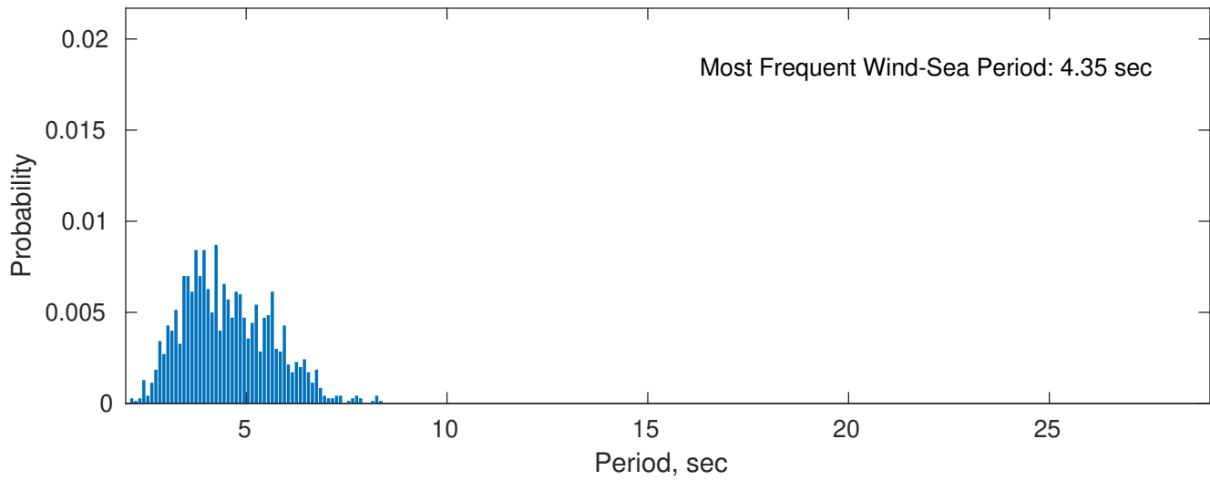
Wind-Sea: 19.19%
