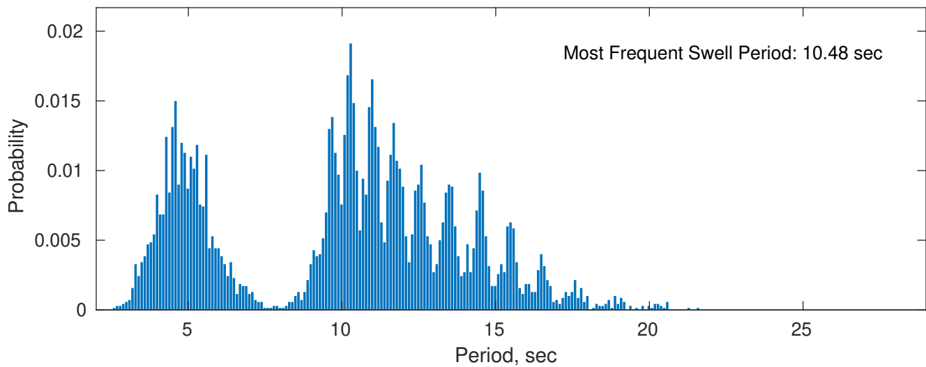
Swell: 80.81%
