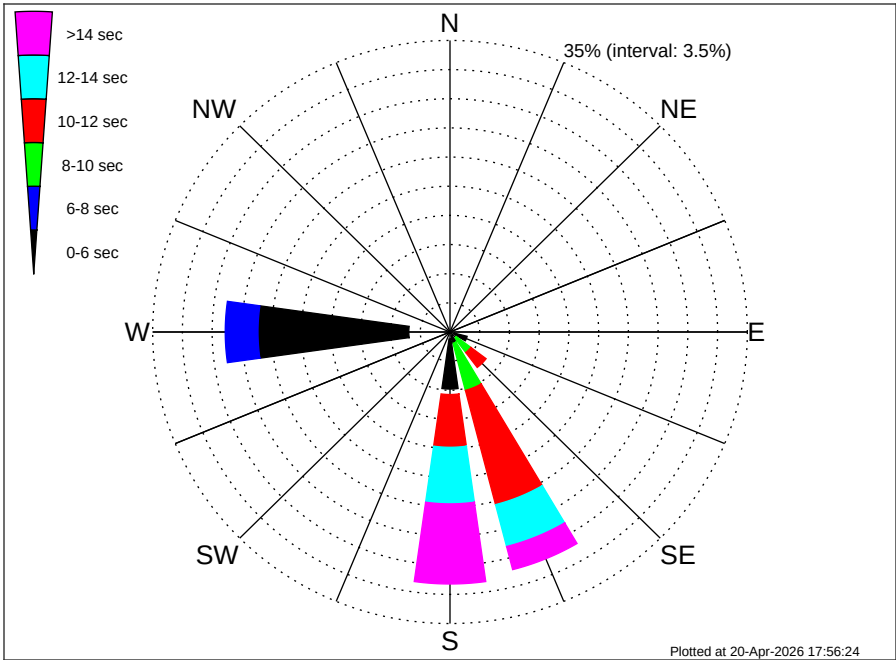
Petronas Oman Block 18 Climatological WavePeriod Rose for February: 1979 - 2015
